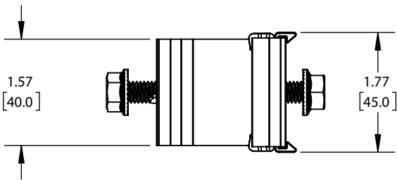
1) CLICKFIT RAIL ATTACHMENT ASSY W/MNT BOLT
