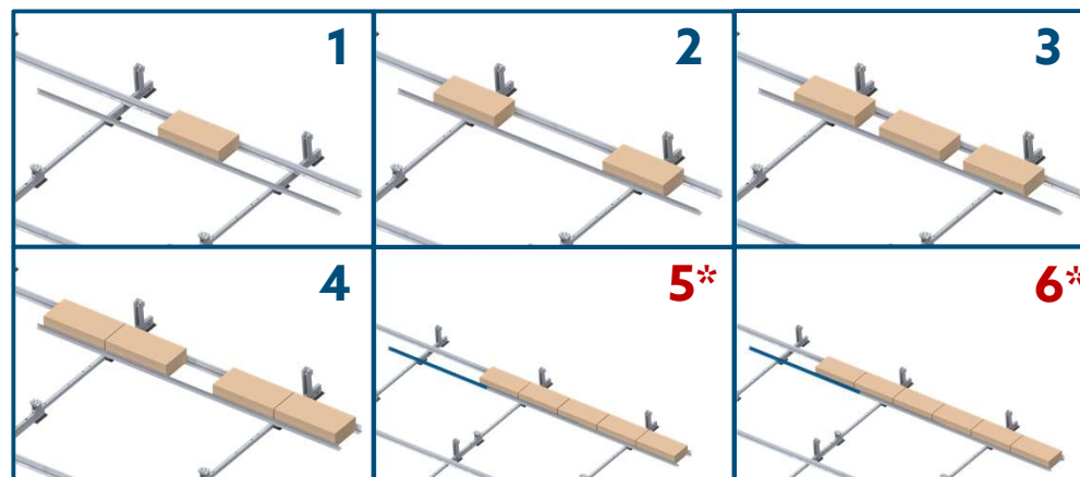
Ballast Positioning for 1-6 Ballast blocks
