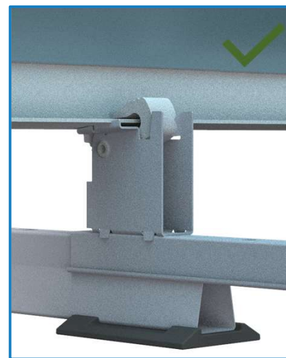
Example of a typical good Cam Claw install, after the module has been rotated down and high-side has been installed
